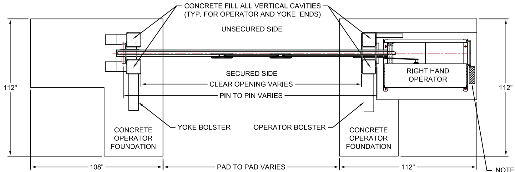
PLAN VIEW
