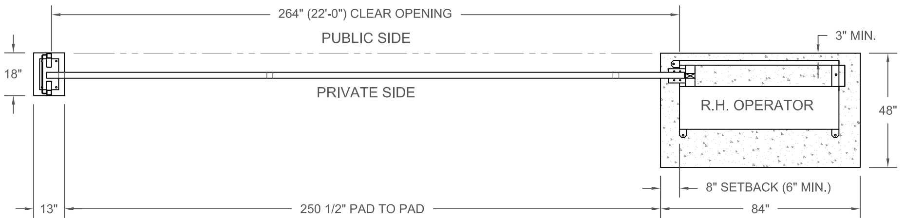
PLAN VIEW
