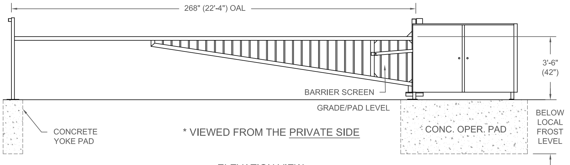
ELEVATION VIEW
